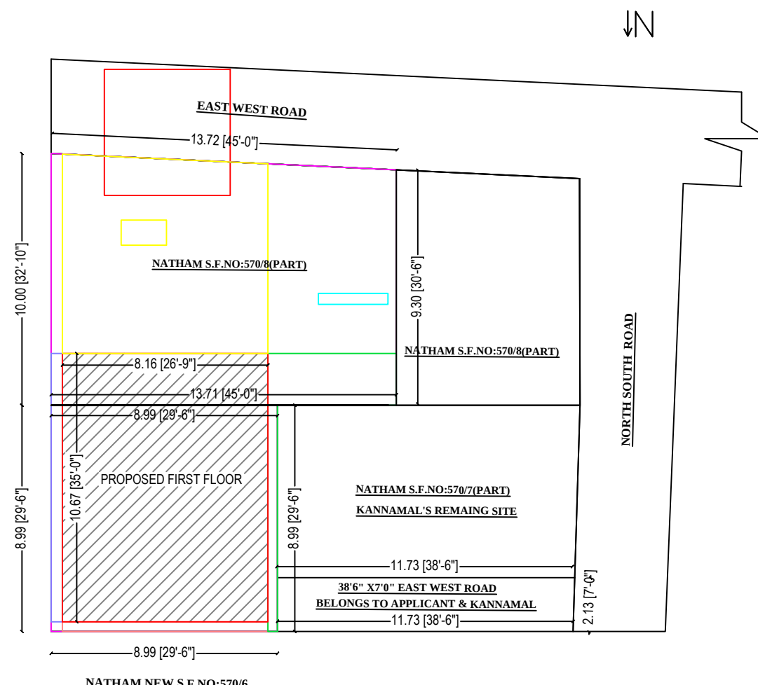
SITE PLAN
