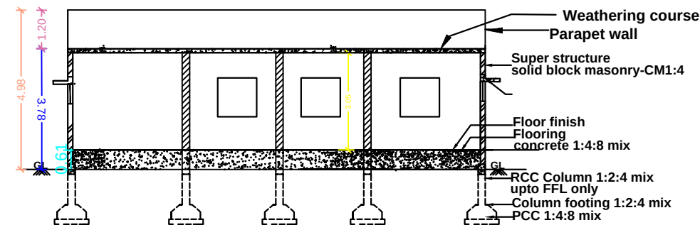
SECTION ELEVATION
