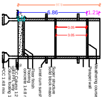
SECTION ELEVATION
