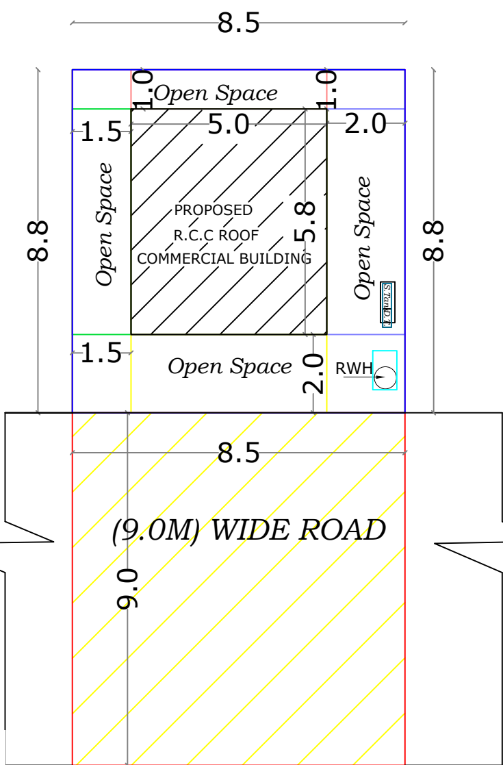
SITE PLAN SUPER IMPOSED PLAN
