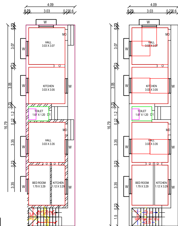
3 GROUND FLOOR BUILDING 39-B-51& PROPOSED ADDITIONAL 1 FLOOR BUILDING
