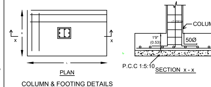
COLUMN & FOOTING DETAILS
