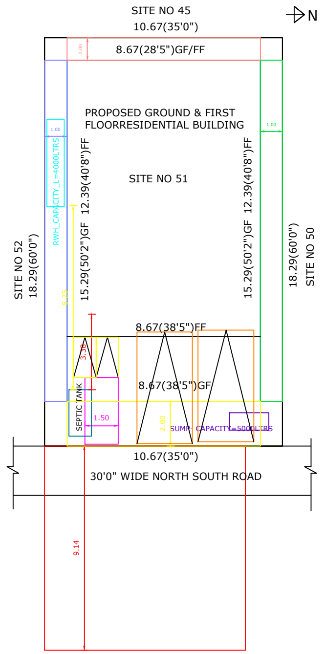
SITE PLAN
