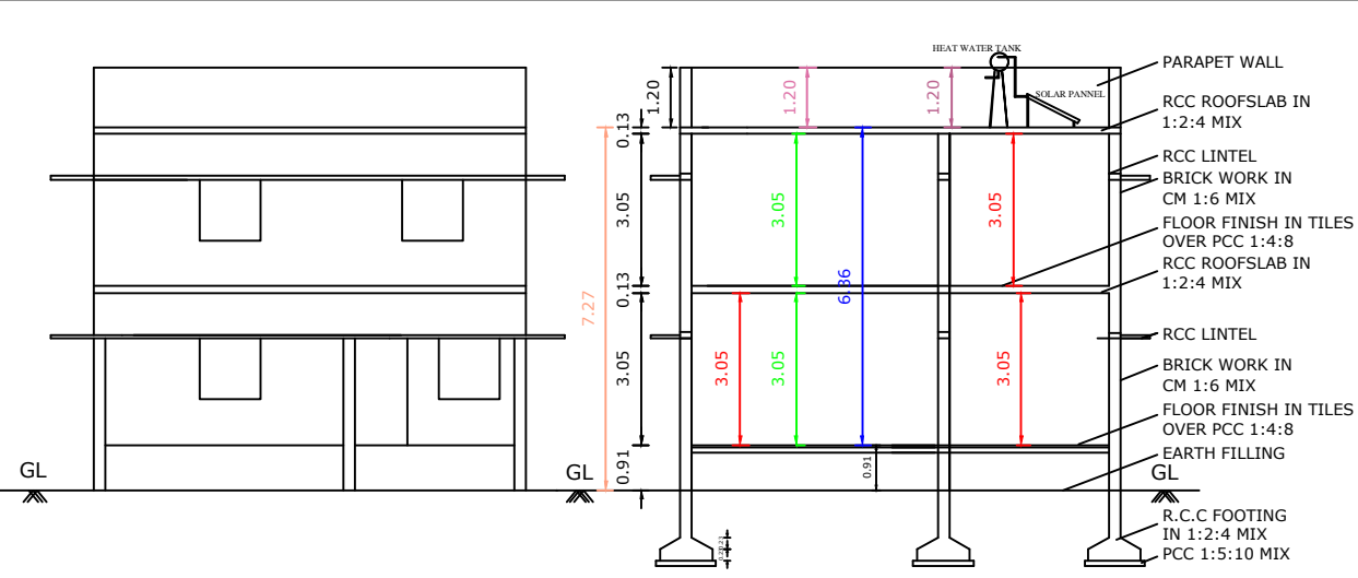
ELEVATION SECTION AA
