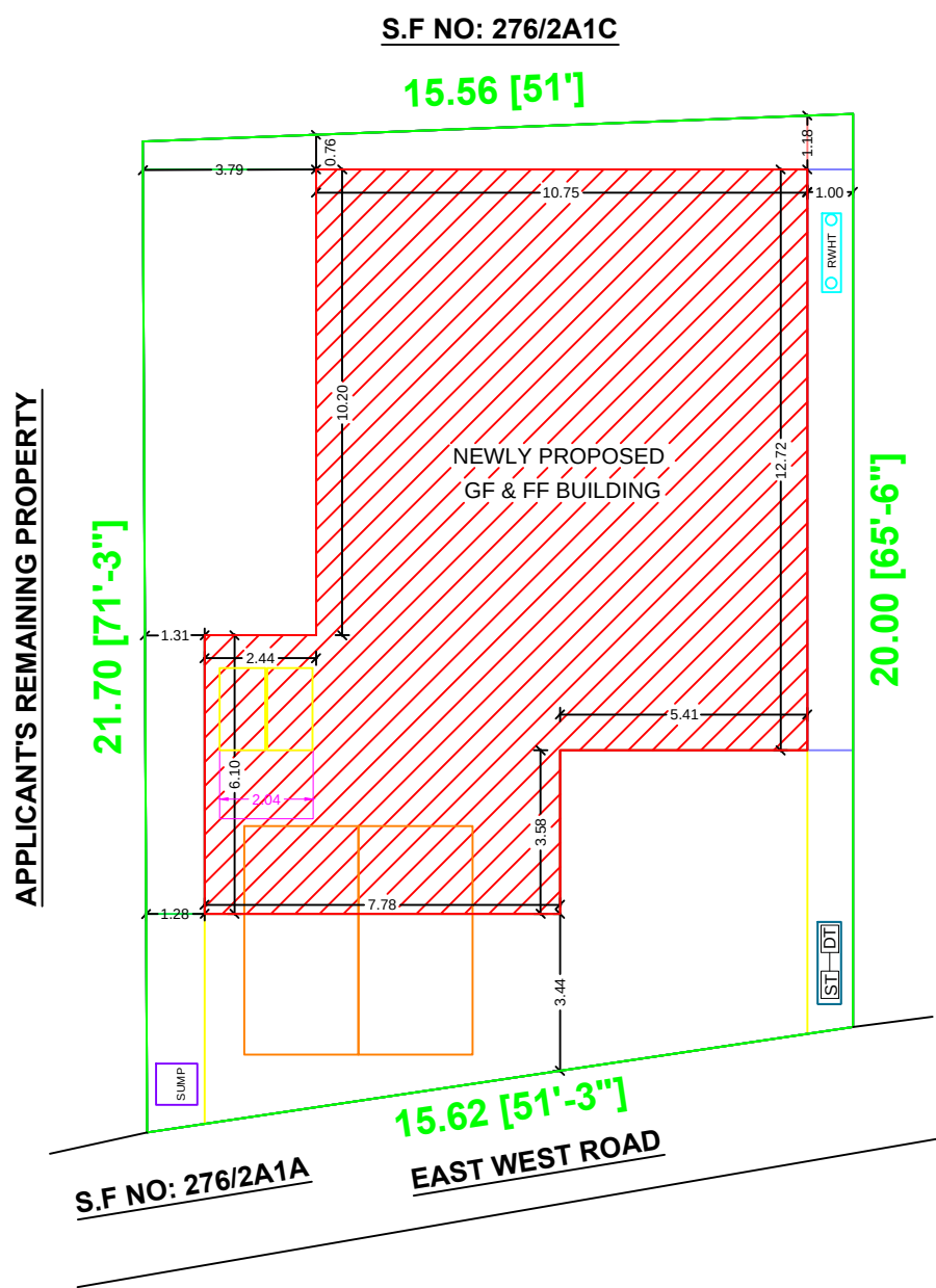
CONCERN SITE PLAN
