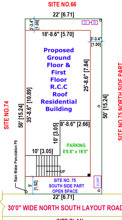
SITE PLAN (SCALE - 1" = 8' 0")
