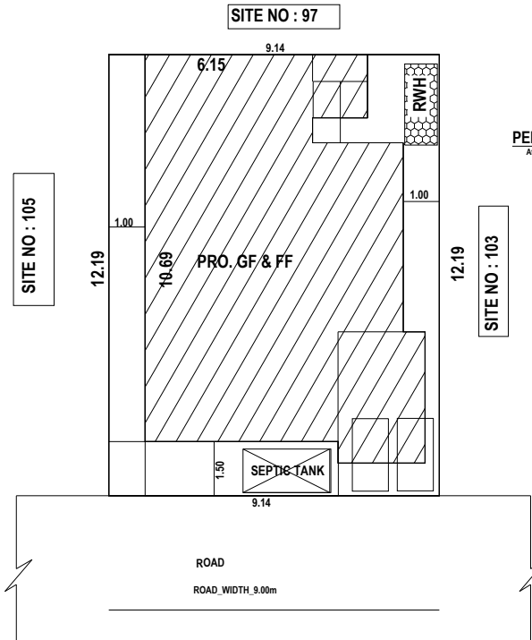
SITE PLAN
