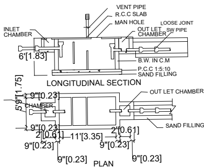
SEPTIC TANK:
