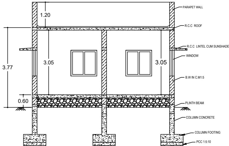
SECTION AB
