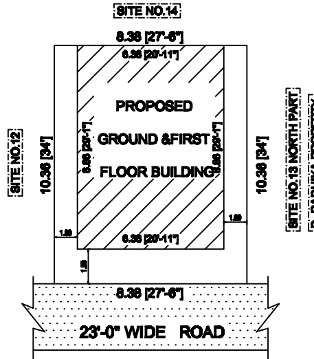
SITE PLAN
