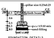
FOUNDATION DETAILS
