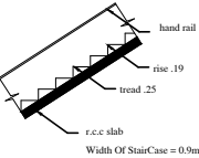
STAIRCASE
