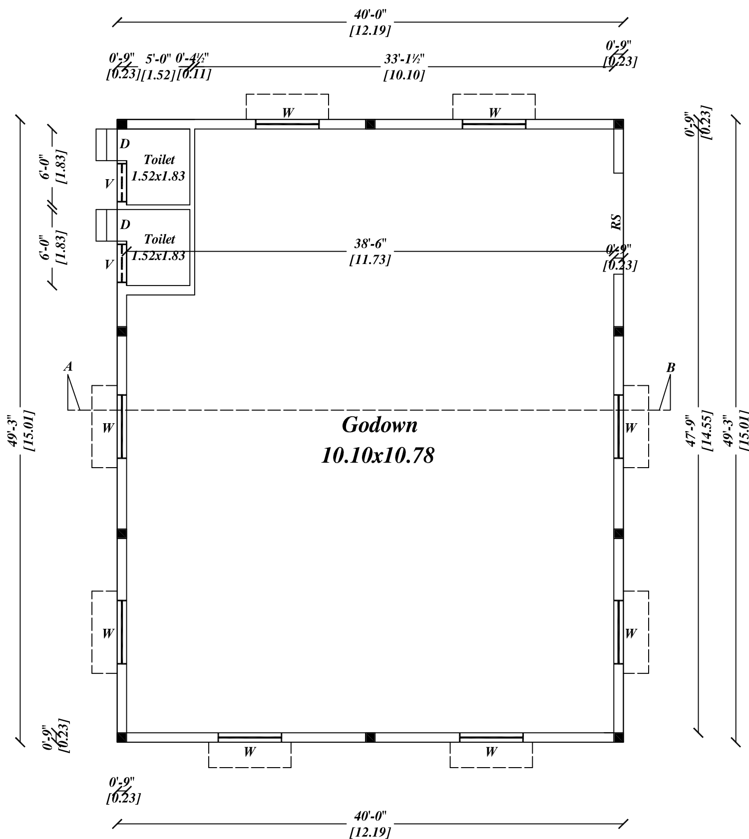
Ground FloorPlan
