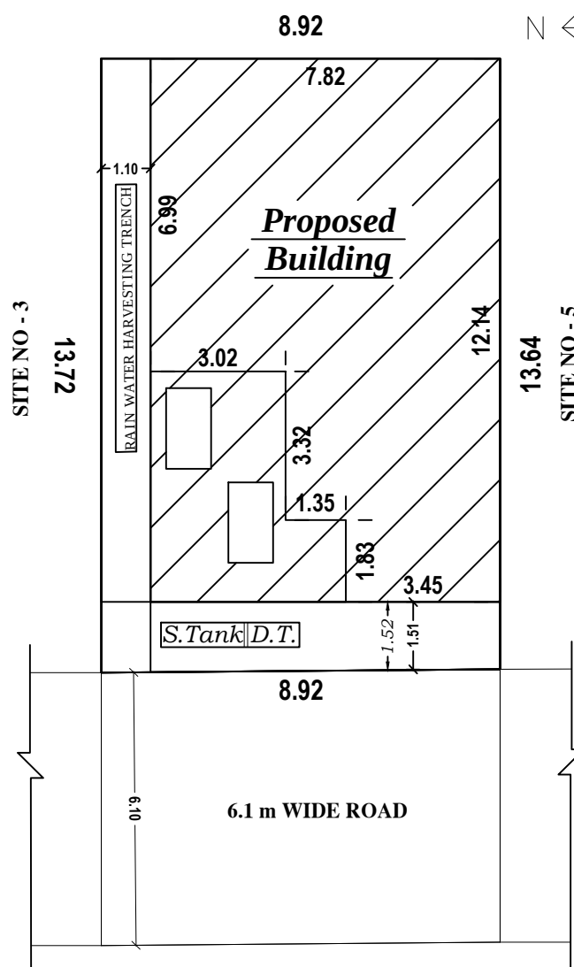
SITE PLAN
