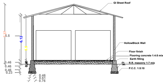
GODOWN BUILDING CROSS SECTION A'-A
