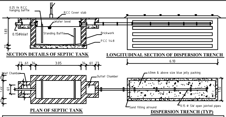
DETAILS OF SEPTIC TANK - 250 GALLONS & DISPERSION TRENCH
