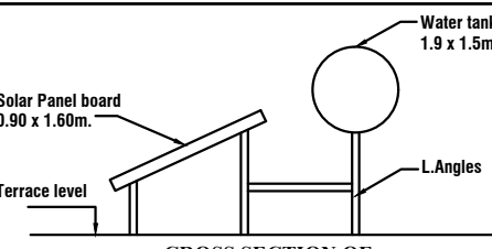
CROSS SECTION OF SOLAR WATER HEATING SYSTEM
