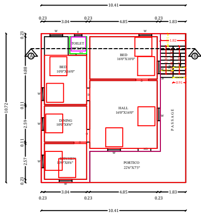
EXISTING ALT.GROUND FLOOR PLAN
