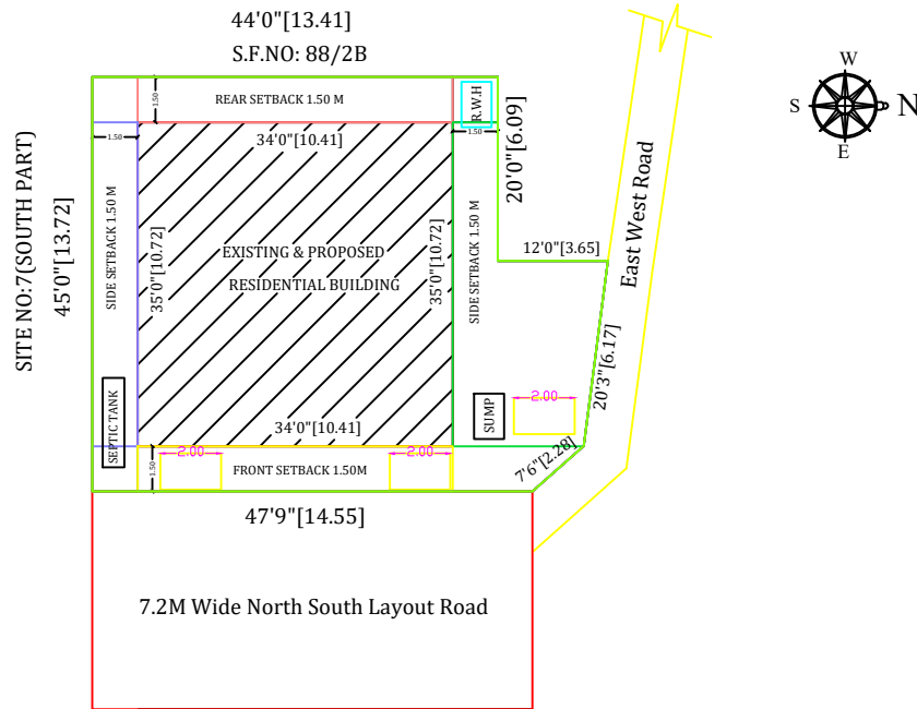
SITE PLAN
