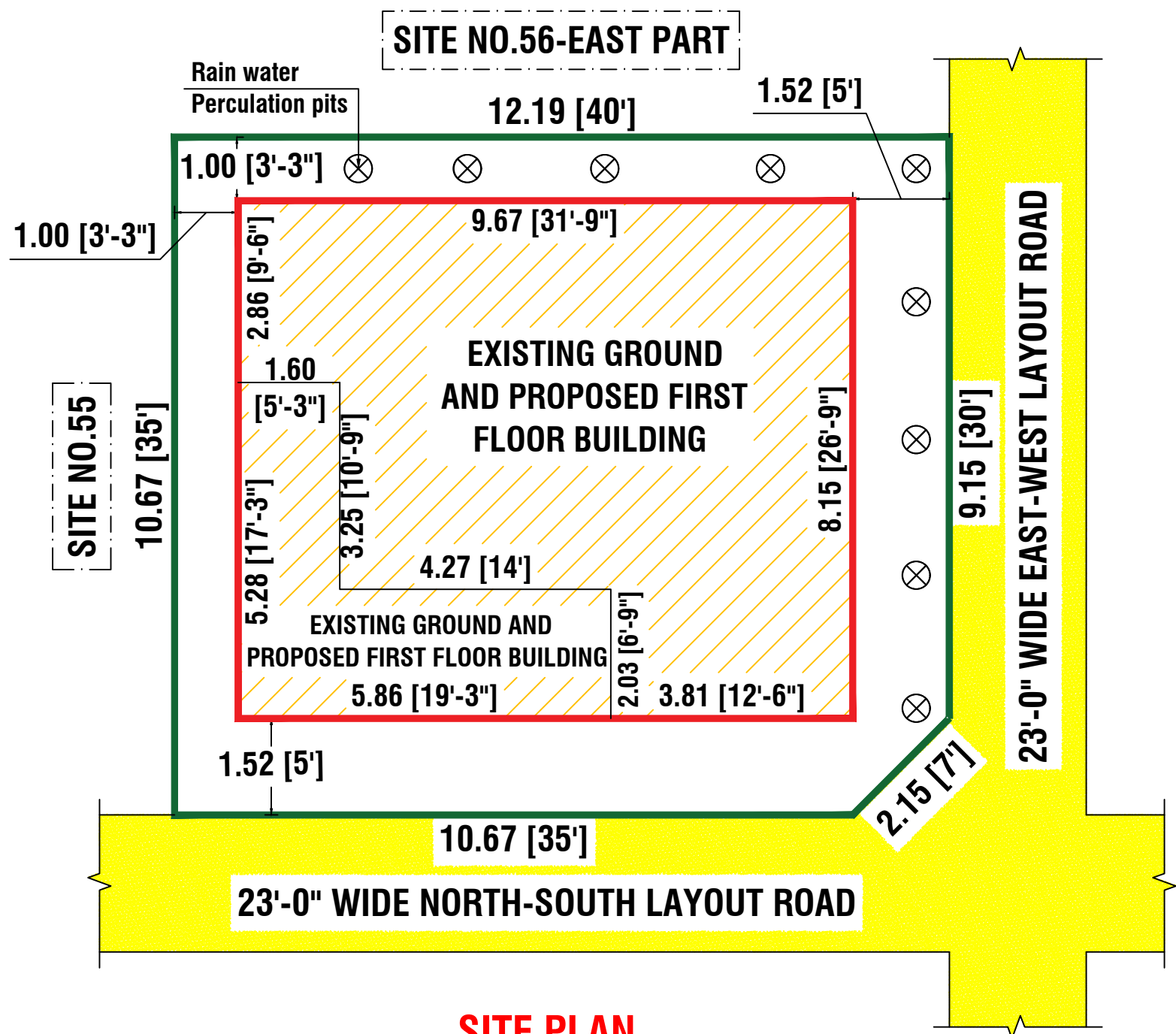
SITE PLAN
