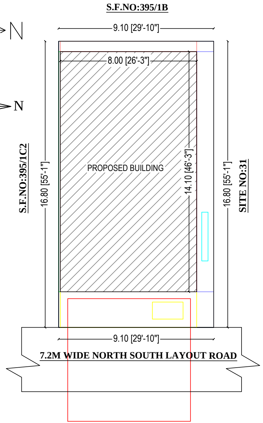
SITE PLAN
