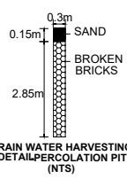
RAIN WATER HARVESTING DETAIL/PERCOLATION PIT (NTS)
