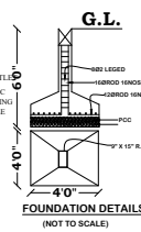
FOUNDATION DETAILS (NOT TO SCALE)
