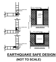
EARTHQUAKE SAFE DESIGN (NOT TO SCALE)
