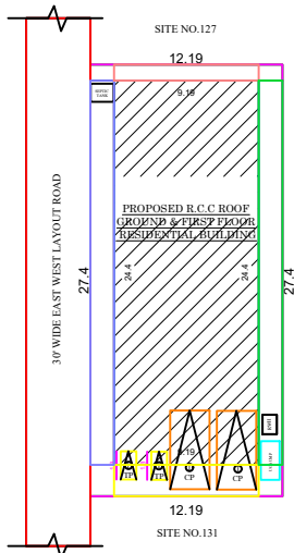
SCALE - 1:100
