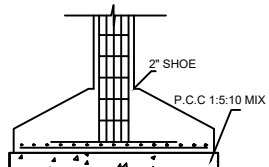
COLUMN DETAIL
