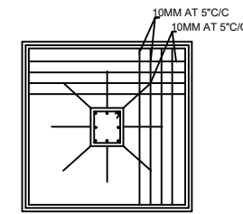
FOOTING DETAIL SCALE: NTS
