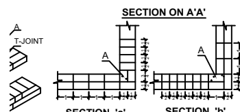
SECTION 'a' SECTION 'b' TYPICAL DETAILS OF PROVIDING VERTICAL STEEL BARS IN BRICK MASONRY
