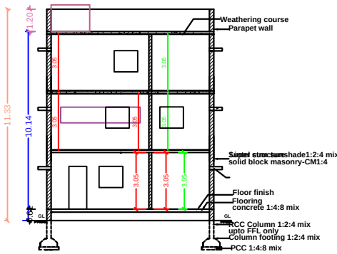
SECTION ELEVATION
