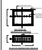
DISPERSION TRENCH
