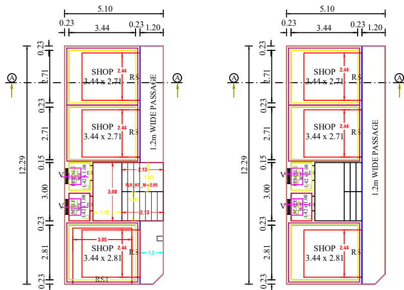
PRO. GROUND FLOOR PLAN
