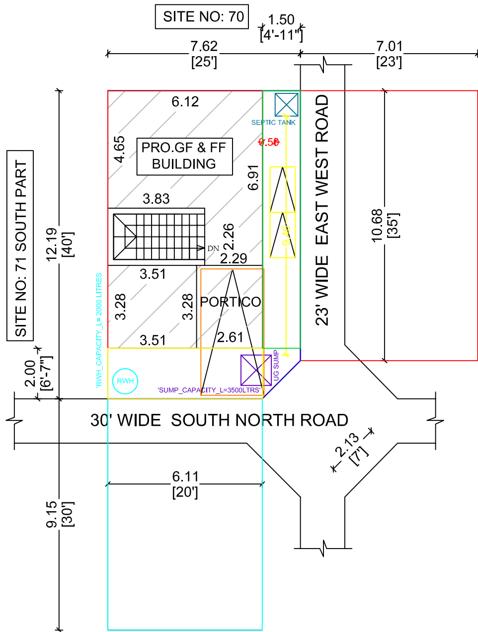
SITE PLAN
