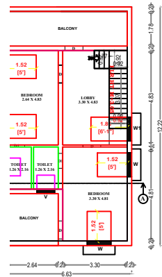
PROPOSED FIRST FLOOR
