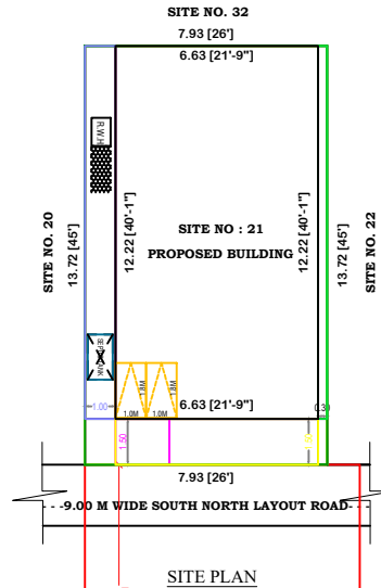
SITE PLAN
