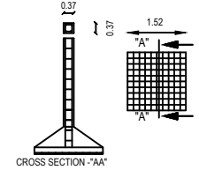
COLUMN DETAILS :-
