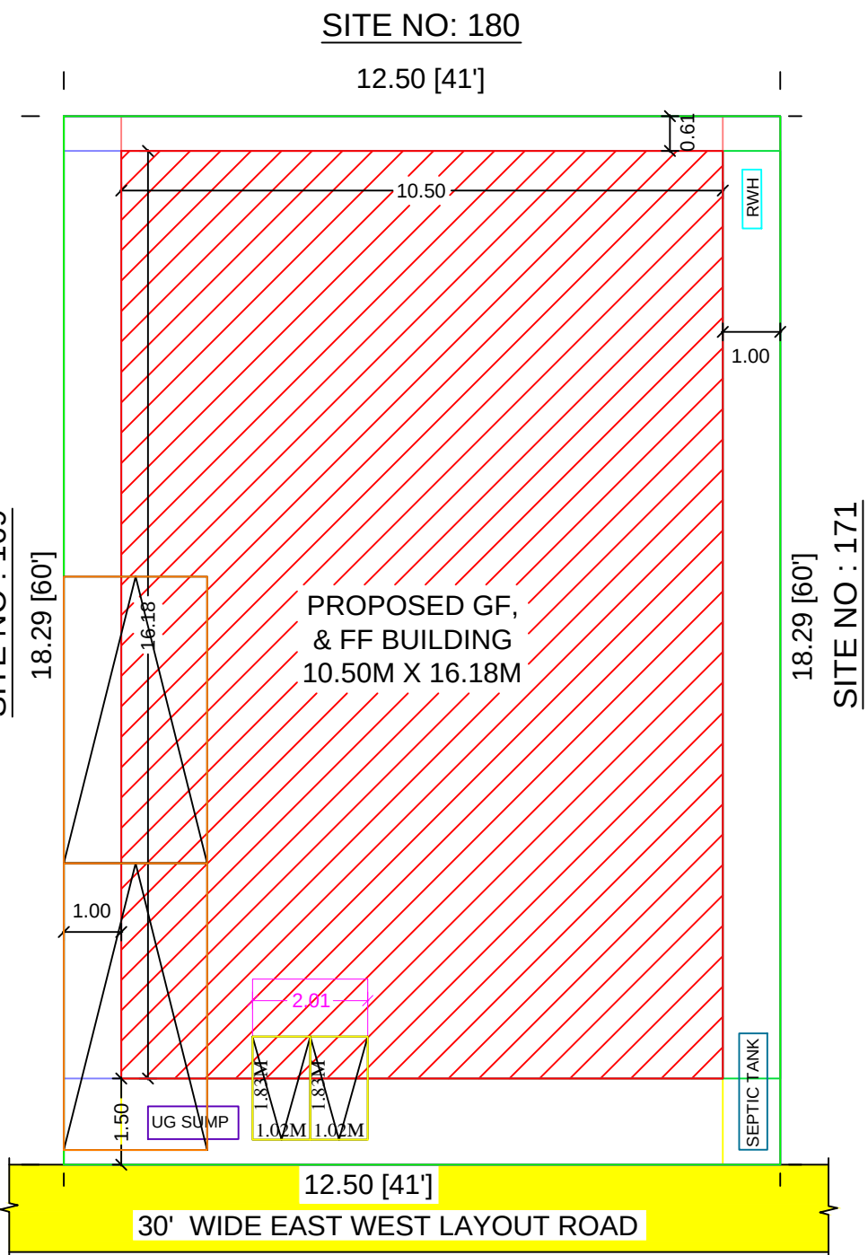
SITE PLAN
