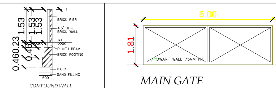
MAIN GATE
