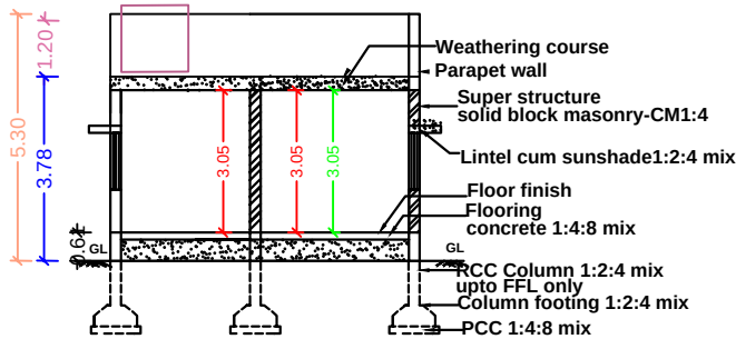
SECTION ELEVATION
