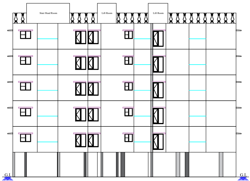
ELEVATION ON EAST SIDE
