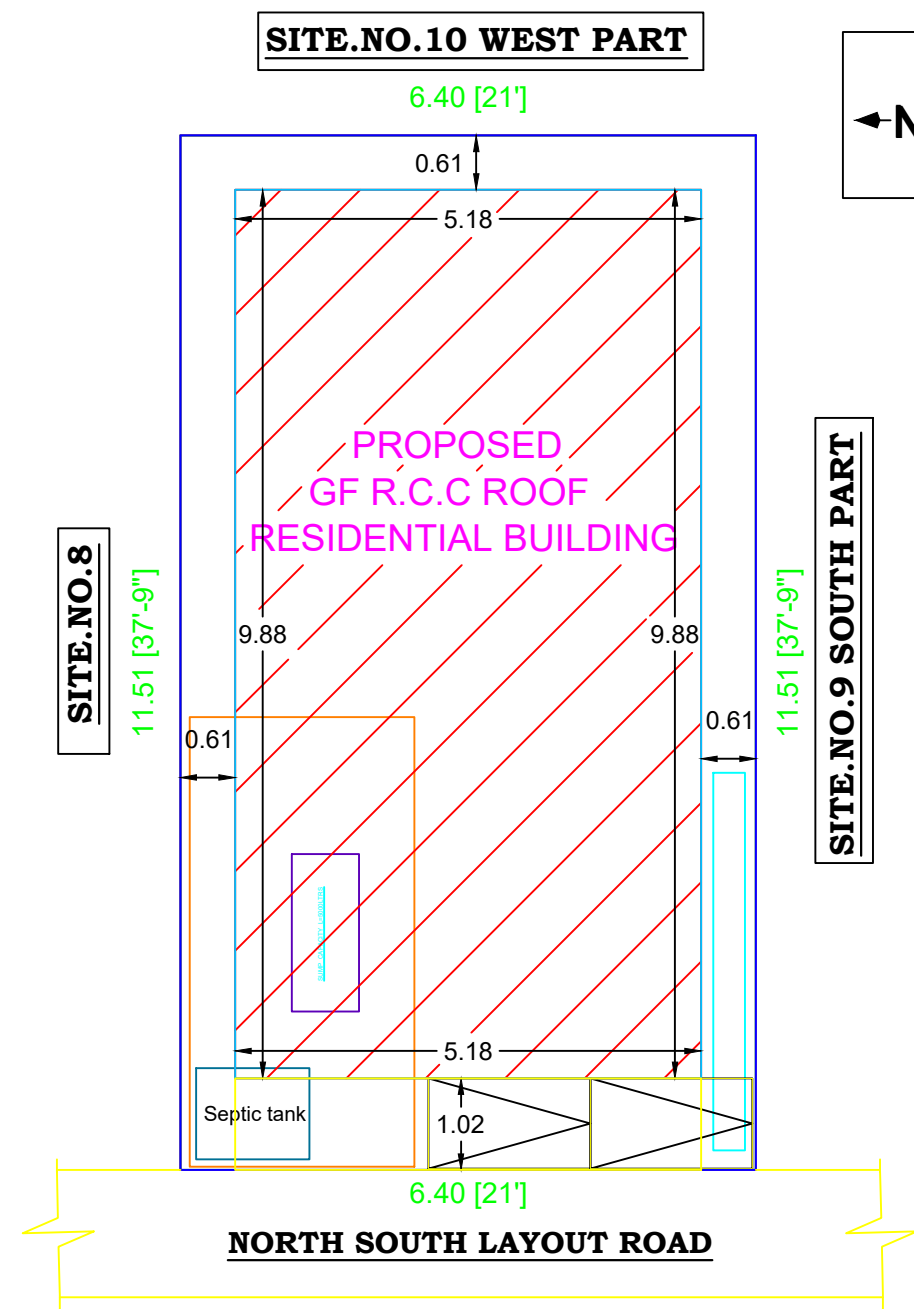
SITE PLAN
