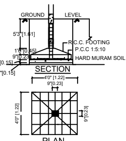
PLAN COLUMN SIZE = 0'9" X 0'9"
