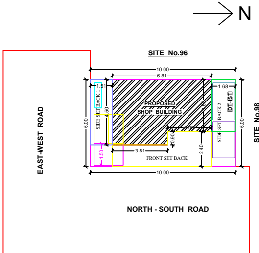
SITE PLAN
