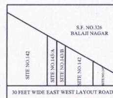
SITE PLAN
