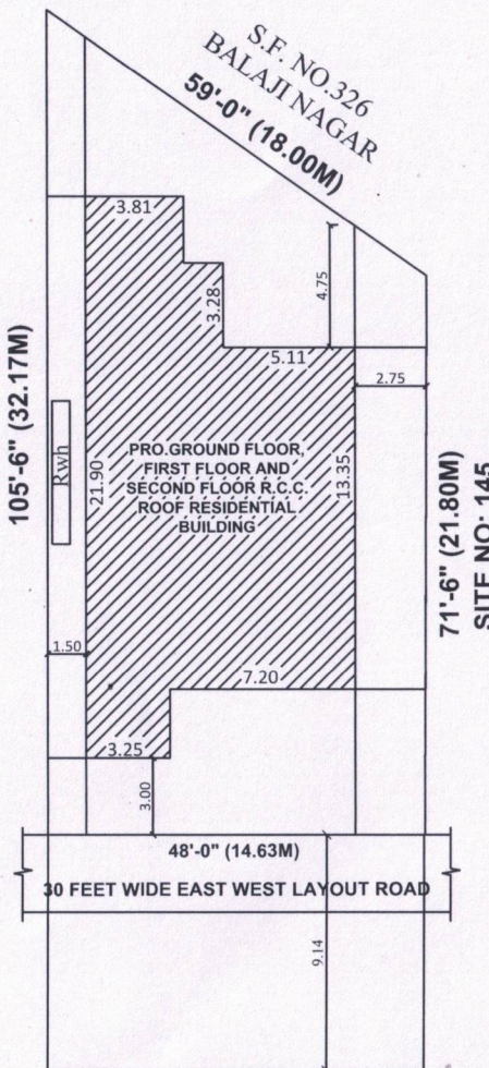
SITE PLAN
