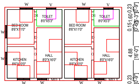
PROPOSED PLAN-2
