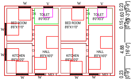
PROPOSED PLAN-1
