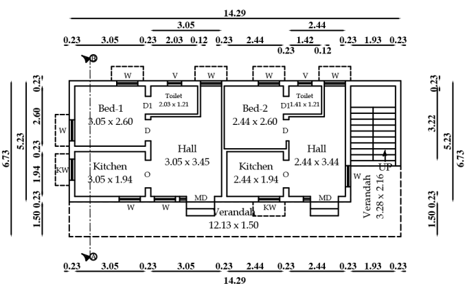
Revised Existing Ground Floor Plan
