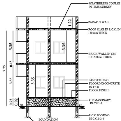
Northern Side Section On "AB"
