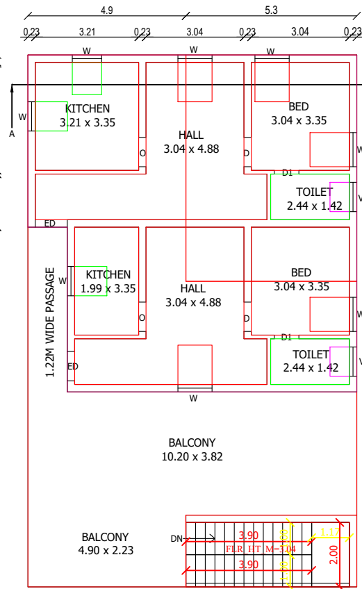
EXISTING & PROPOSED FIRST FLOOR PLAN
