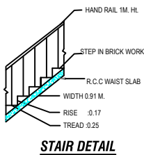
STAIR DETAIL
