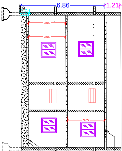
SECTION ELEVATION
