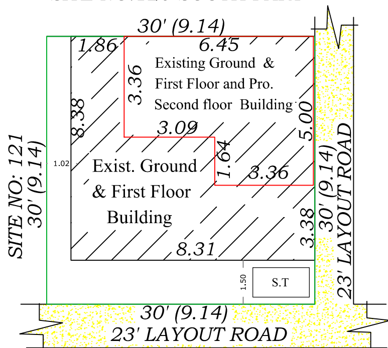
SITE PLAN
