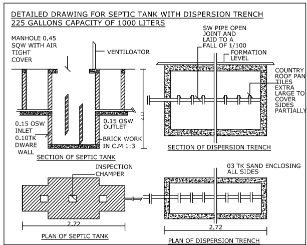
SITE NO:120 SOUTH PART
