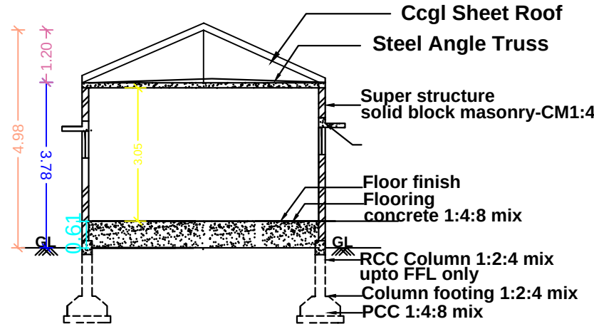
SECTION ELEVATION
