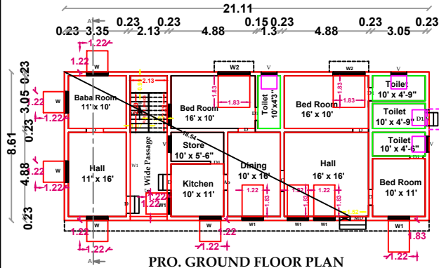
PRO. GROUND FLOOR PLAN
