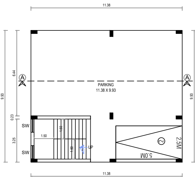
STILT FLOOR PLAN
