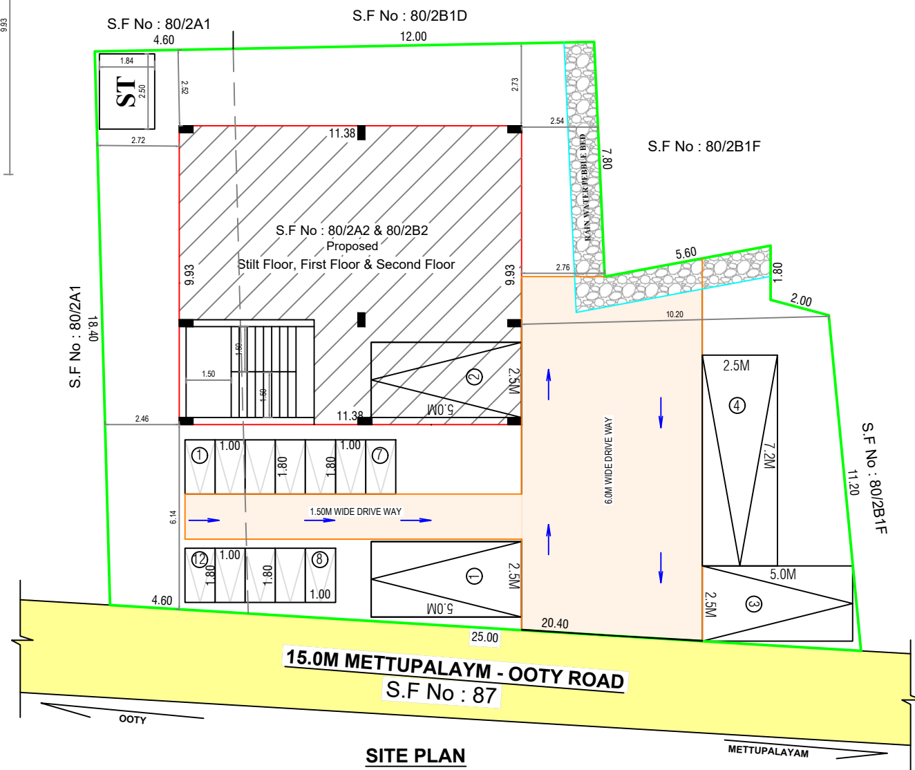
SITE PLAN
