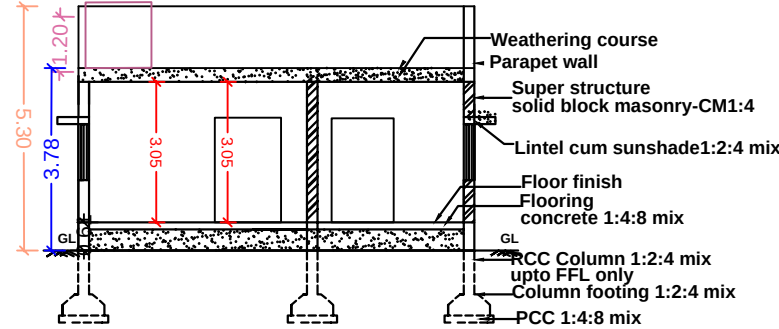
SECTION ELEVATION
