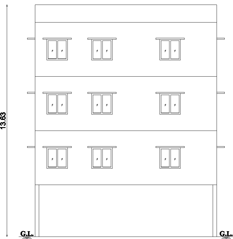
EAST ELEVATION
