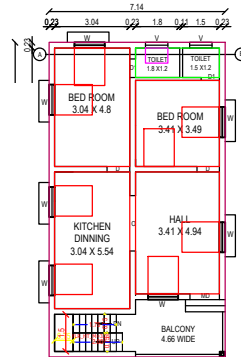
PROPOSED ADDITIONAL FIRST FLOOR BUILDING
