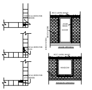
EARTHQUAKE SAFE DESIGN (NOT TO SCALE)
