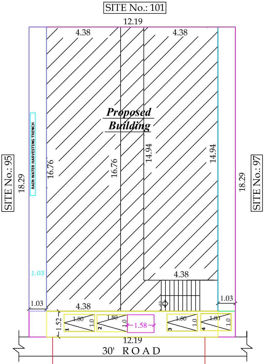
SITE PLAN
