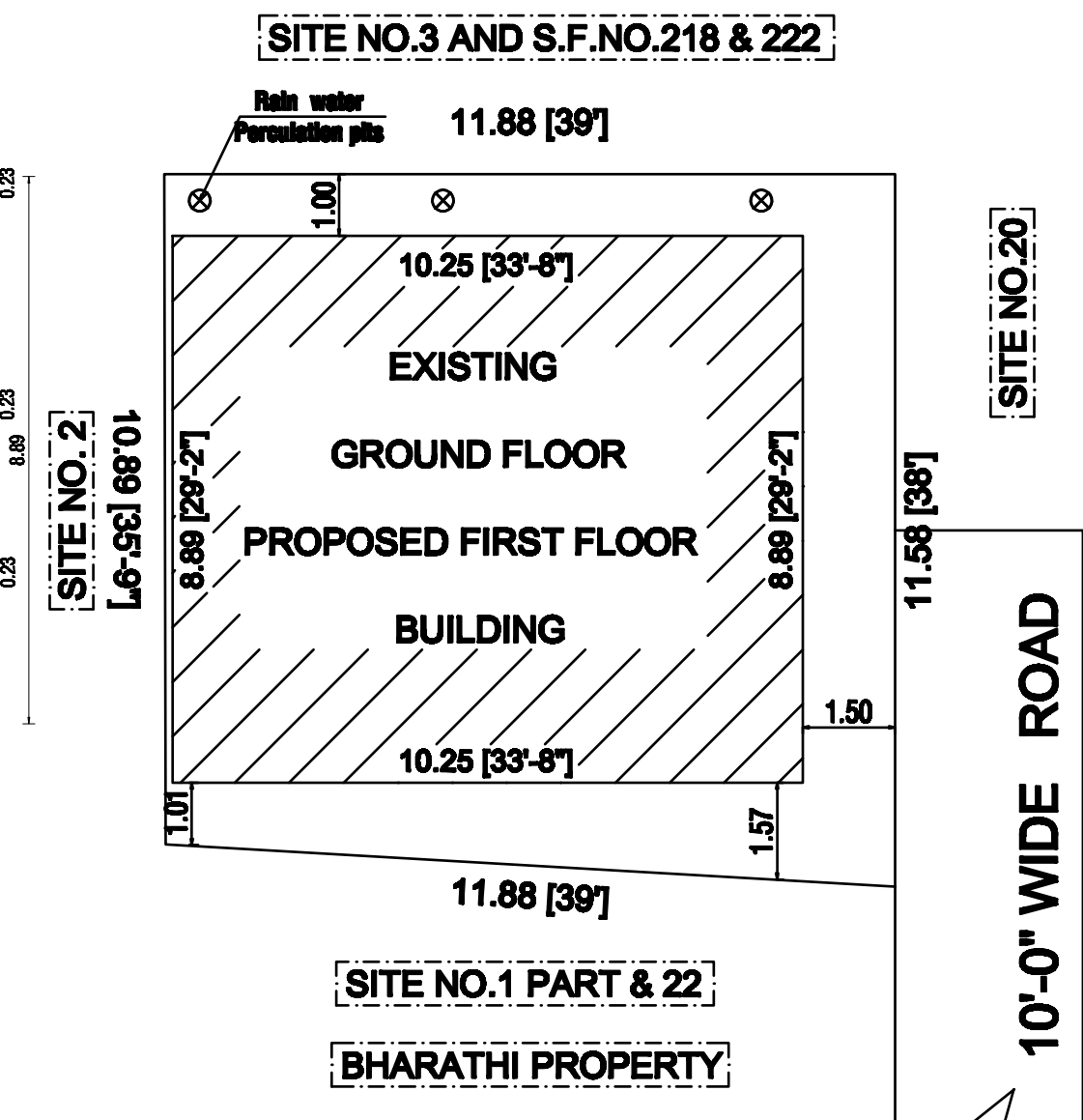
SITE PLAN
